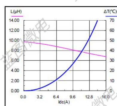
SMS1360-100M
