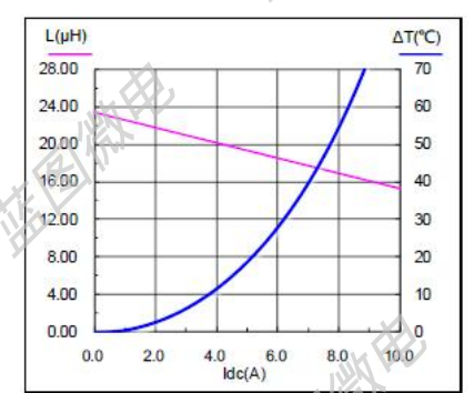
SMS1360-220M
