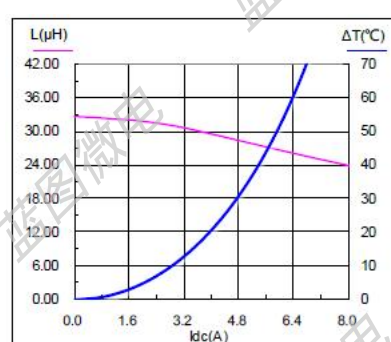
SMS1360-330M
