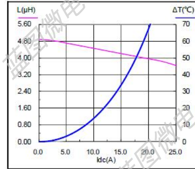
SMS1360-100M
