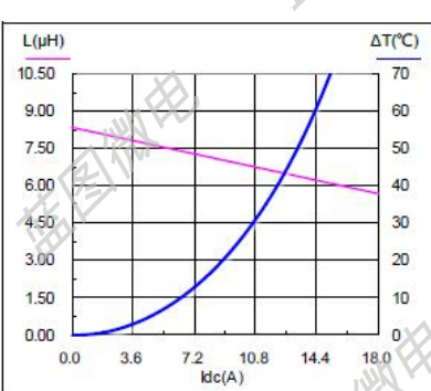
SMS1360-8R2M
