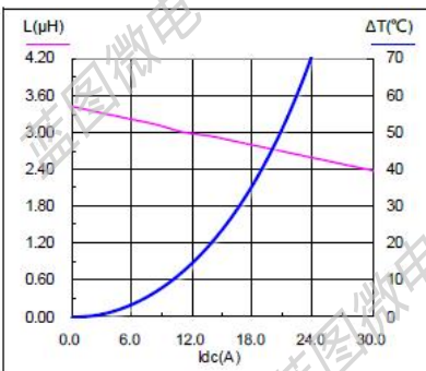
SMS1360-8R2M
