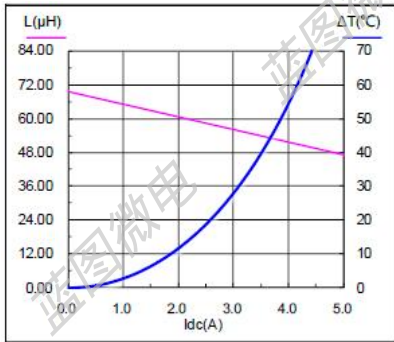
SMS1360-680M
