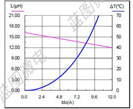
SMS1350-150M
