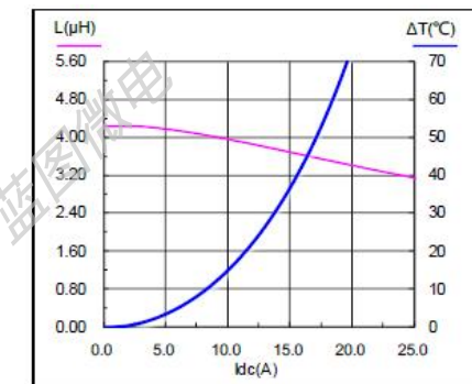
SMS1350-4R7M
