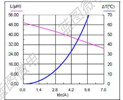
SMS1350-470M
