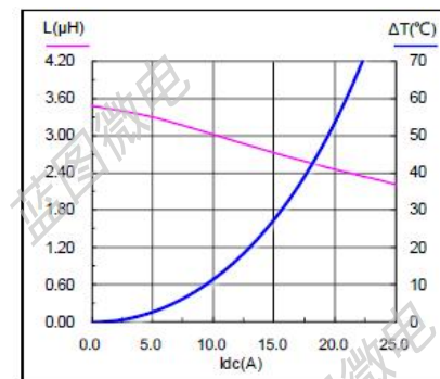
SMS1350-3R3M
