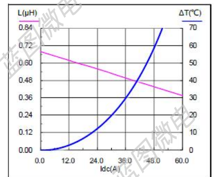
SMS1350-1R5M
