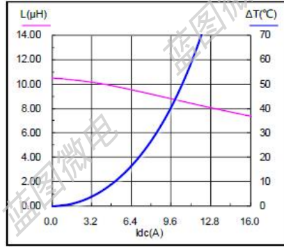
SMS1350-100M
