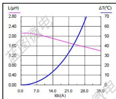
SMS1350-2R2M
