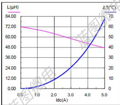
SMS1350-680M
