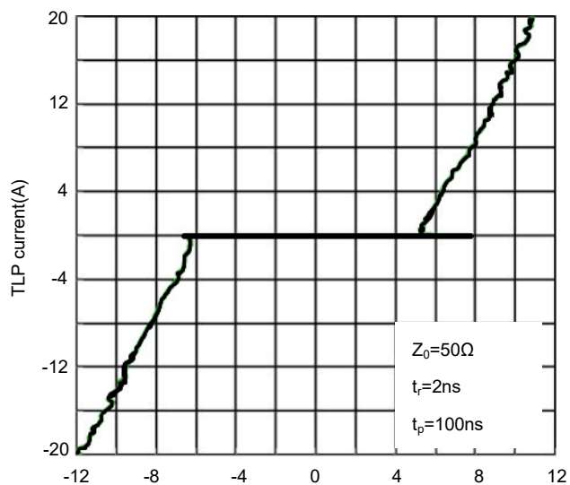
Fig 7 TLP Measurement
