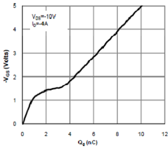
Figure 7: Gate-Charge Characteristics
