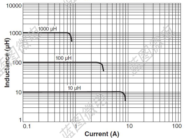
Inductance vs Current
