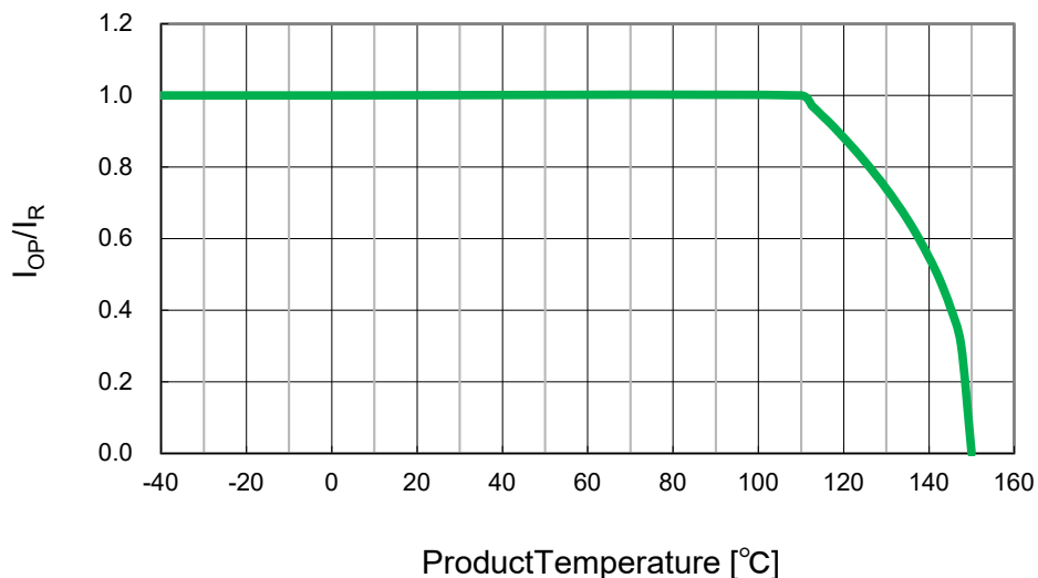
Derating of Rated Current
