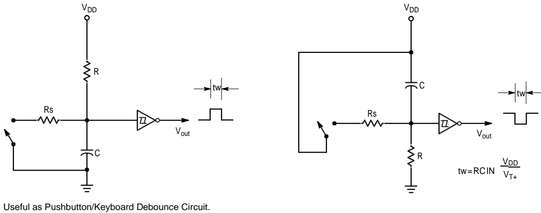
Figure 4. Monostable Multivibrator
