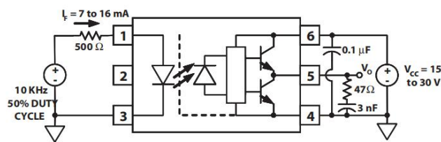
Figure 17. Propagation Delay Test Circuit and Waveforms.
