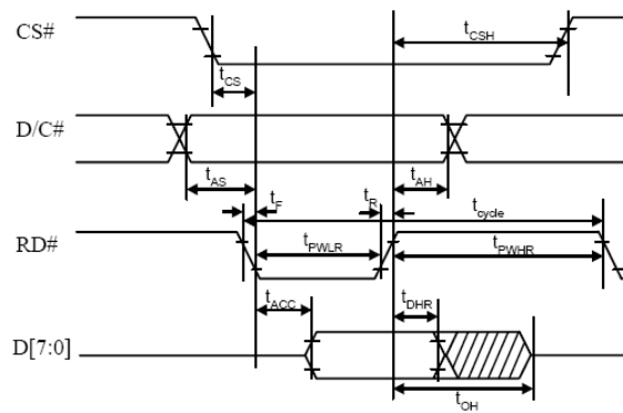
( Read Timing )
