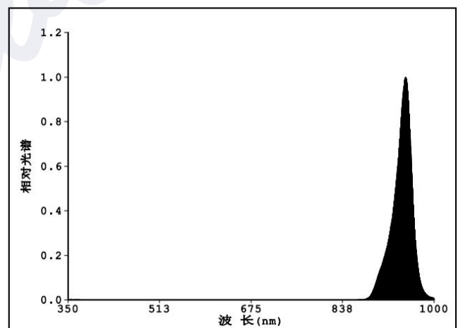
Spectral wavelength
