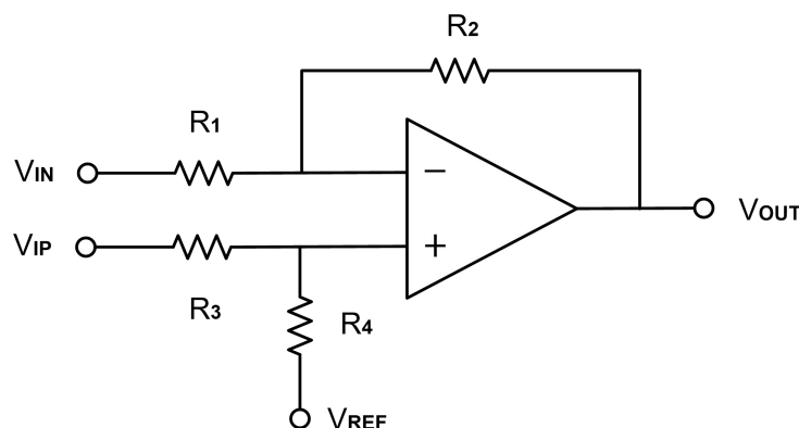
Figure 4. Differential Amplifier
