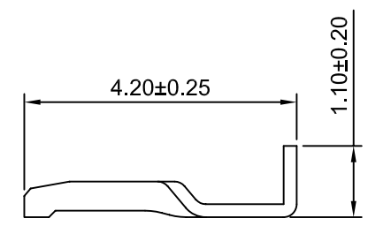
SEC:C-C
