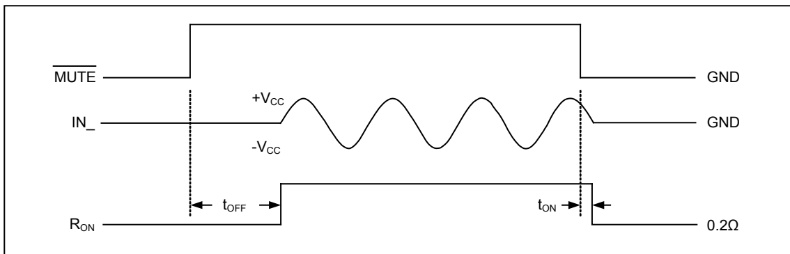
Figure 2. Turn-On/Off Time
