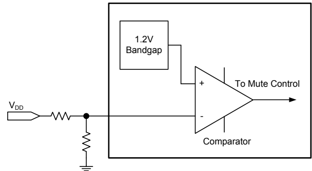
Figure 3. UVP Detection
