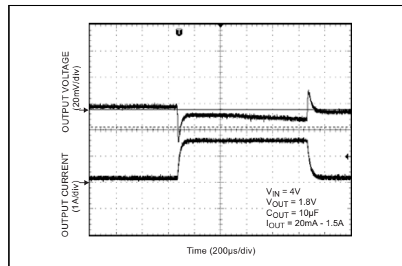
FIGURE 2-12: Load Transient.
