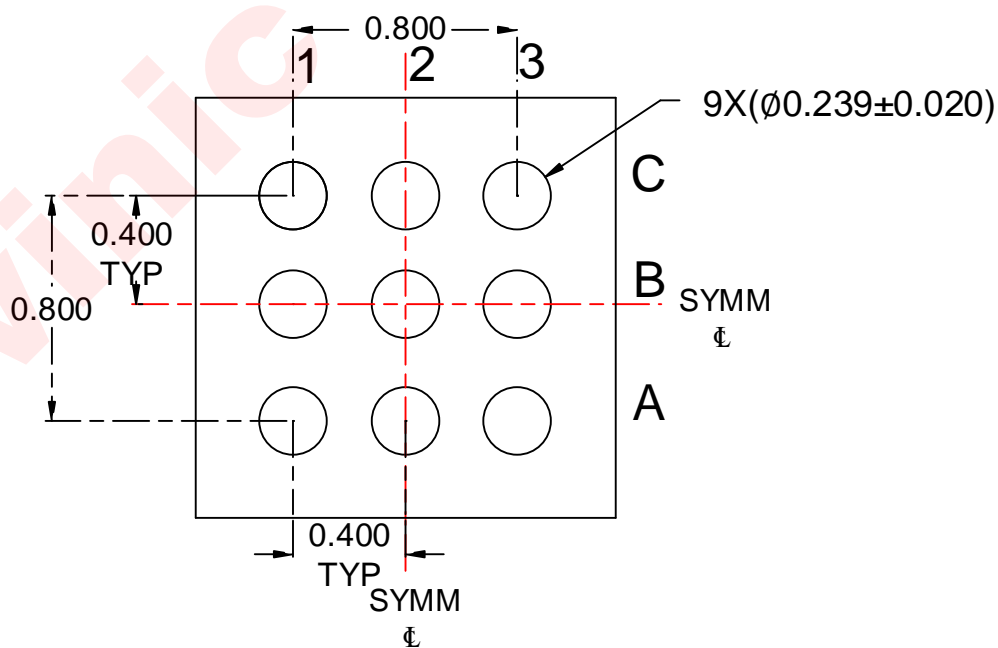
Bottom View
