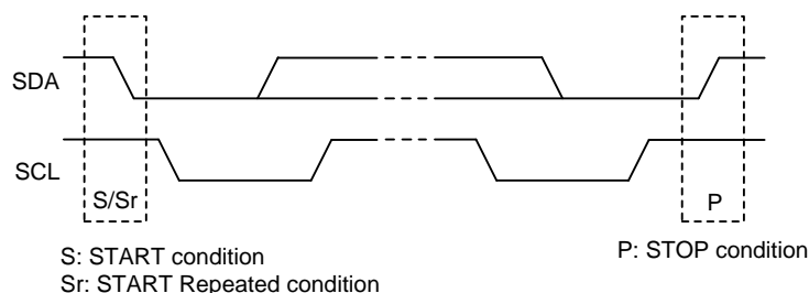
Figure 6. I²C Start/Stop Condition Timing
