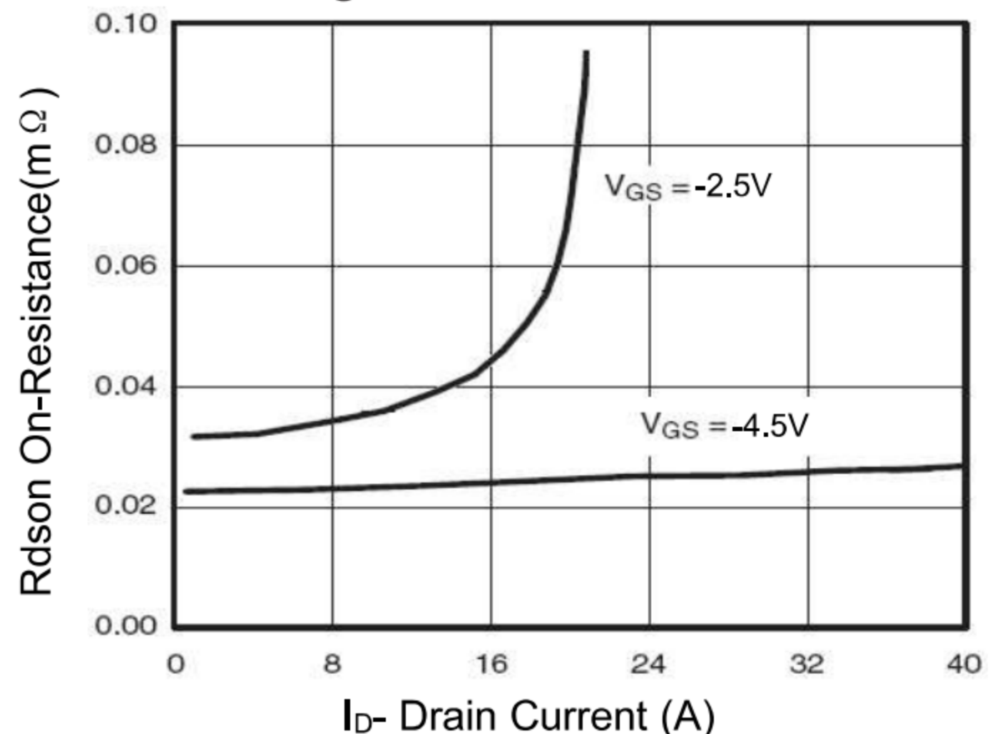
Figure 6 Drain-Source On-Resistance
