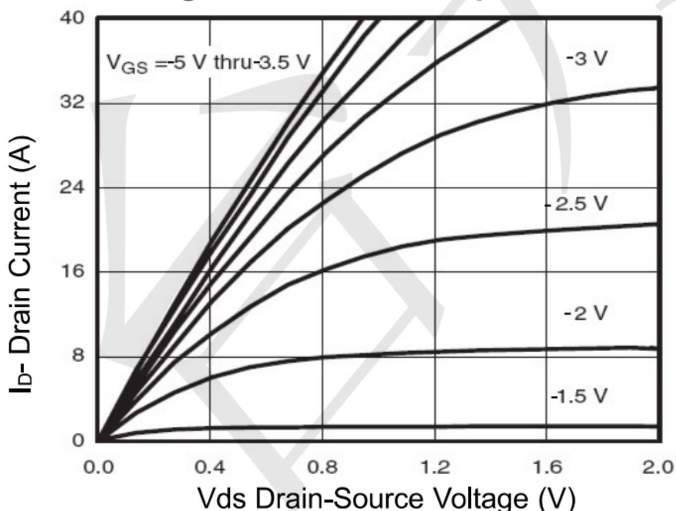
Figure 5 Output Characteristics
