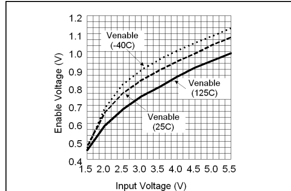
FIGURE 2-4: MIC94040/1 Enable Threshold vs. Input Voltage.
