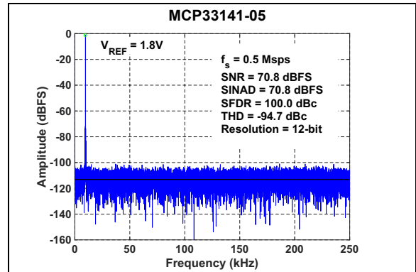
FIGURE 3-12: FFT for 10 kHz Input Signal: f_S = 500\text{ ksp/s} , V_{IN} = -1\text{ dBFS} , V_{REF} = 1.8\text{V} .
