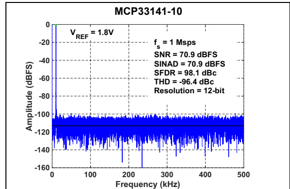
FIGURE 3-11: FFT for 10 kHz Input Signal: f_S = 1\text{ Msp/s} , V_{IN} = -1\text{ dBFS} , V_{REF} = 1.8\text{V} .
