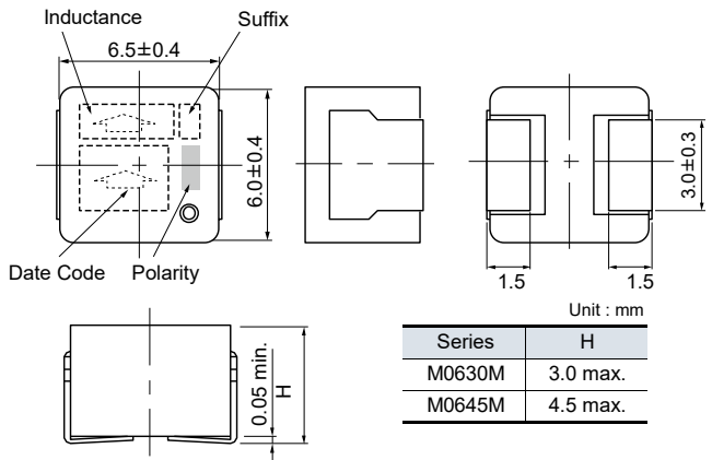
Series PCC-M0630M Series PCC-M0645M (ETQP3M□□□YFN/ETQP4M□□□YFN)
