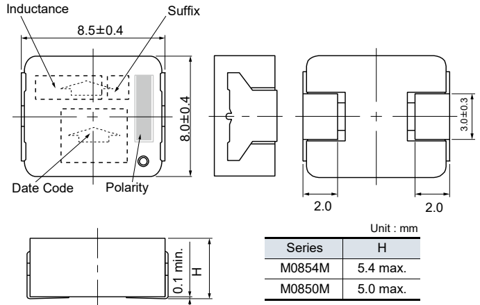
Series PCC-M0854M Series PCC-M0850M (ETQP5M□□□YFK/YGK)
