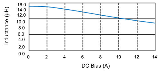
[ ETQP6M150KLC ]
