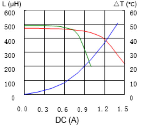
CDRH127LDNP-471MC
