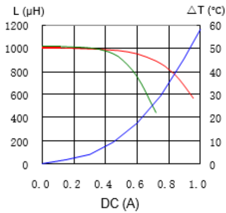
CDRH127LDNP-102MC
