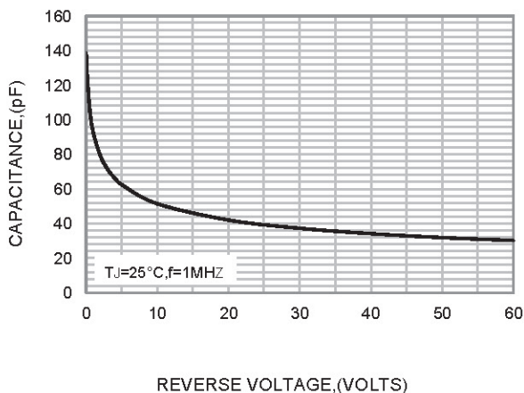
FIG.3-TYPICAL JUNCTION CAPACITANCE
