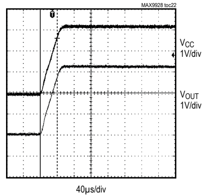
POWER-UP DELAY
