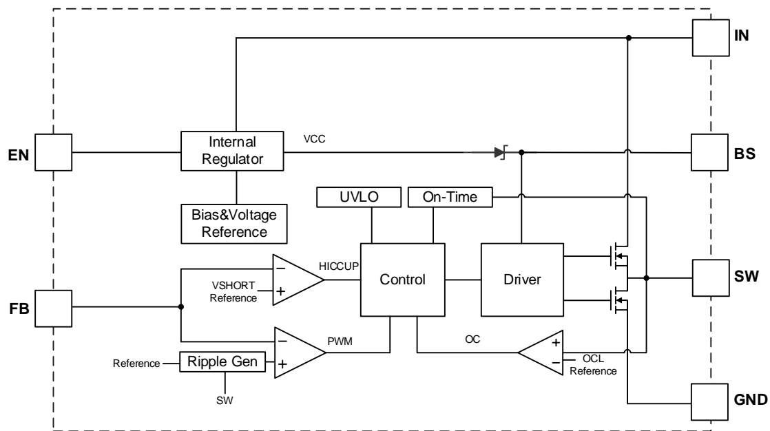
Block Diagram
