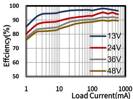
Efficiency (%) VOUT=12V
