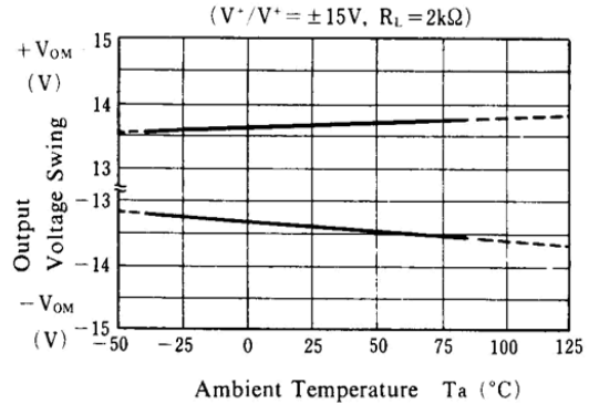
Output Voltage Swing vs. Temperature
