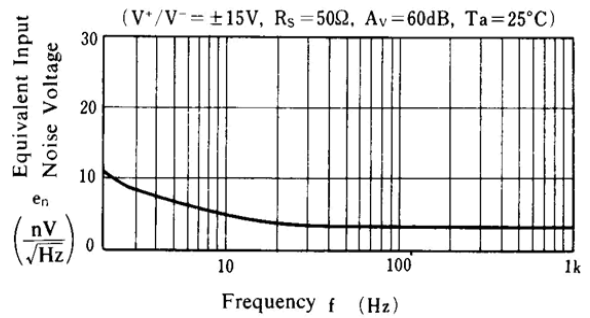
Equivalent Input Noise Voltage vs. Frequency
