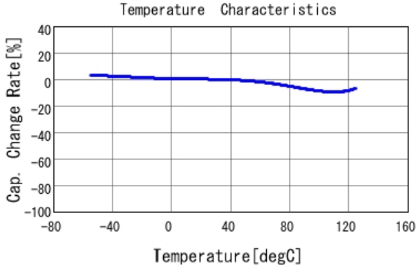
GCM155R71H332KA37 C-Temp. capchange, DC0.0V, AC1.C
