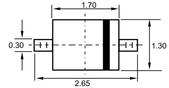
SOD-323
