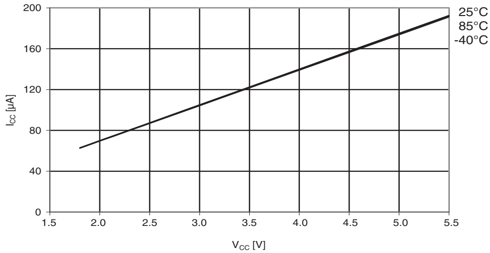
Figure 30-43. ATmega164A: AREF external reference current vs. V_{CC}
