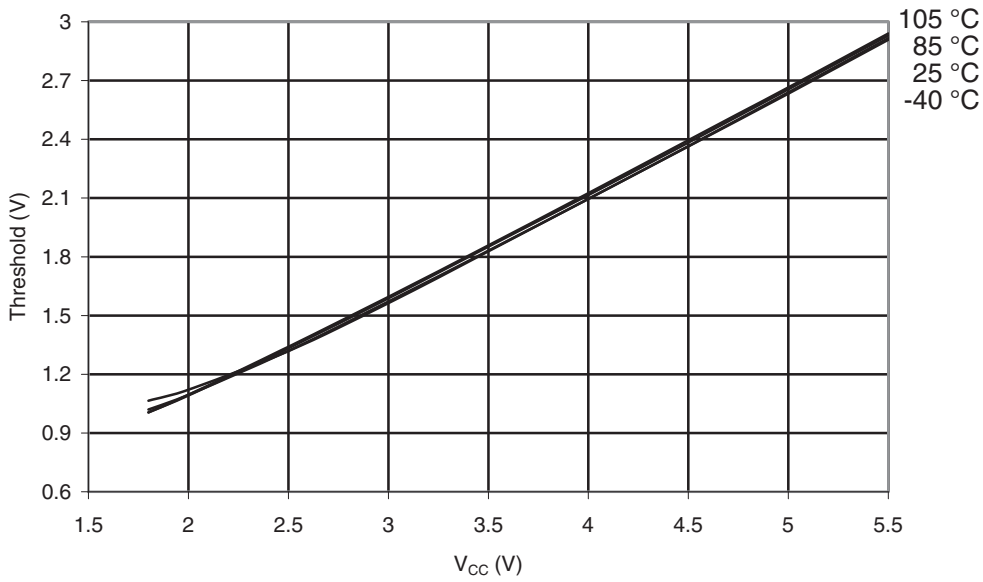
Figure 31-99. I/O Pin Input Threshold vs. V_{CC} ( V_{IH} , I/O Pin Read as '1')
