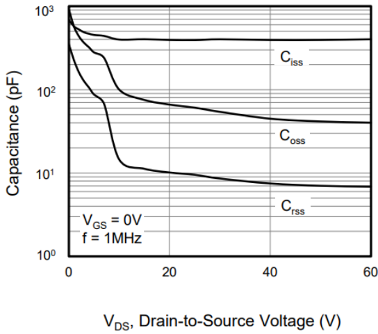
Figure 7. Capacitance
