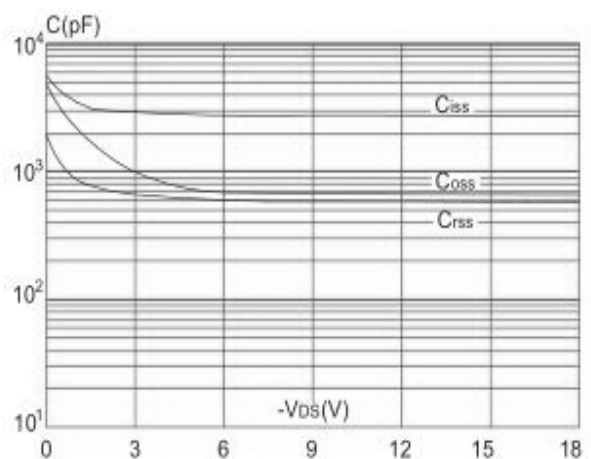
Figure 6: Capacitance Characteristics
