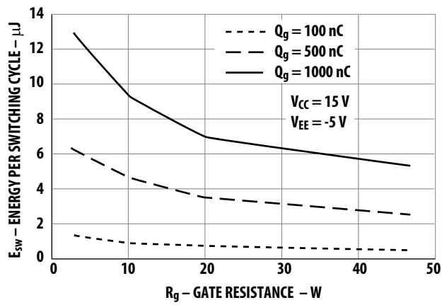
Figure 25 Energy Dissipated in the ACNT-H313 for Each IGBT Switching Cycle
