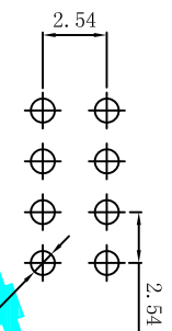
PCB Layout
