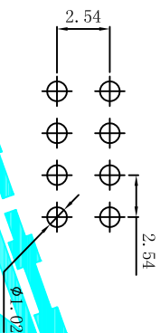
PCB Layout
