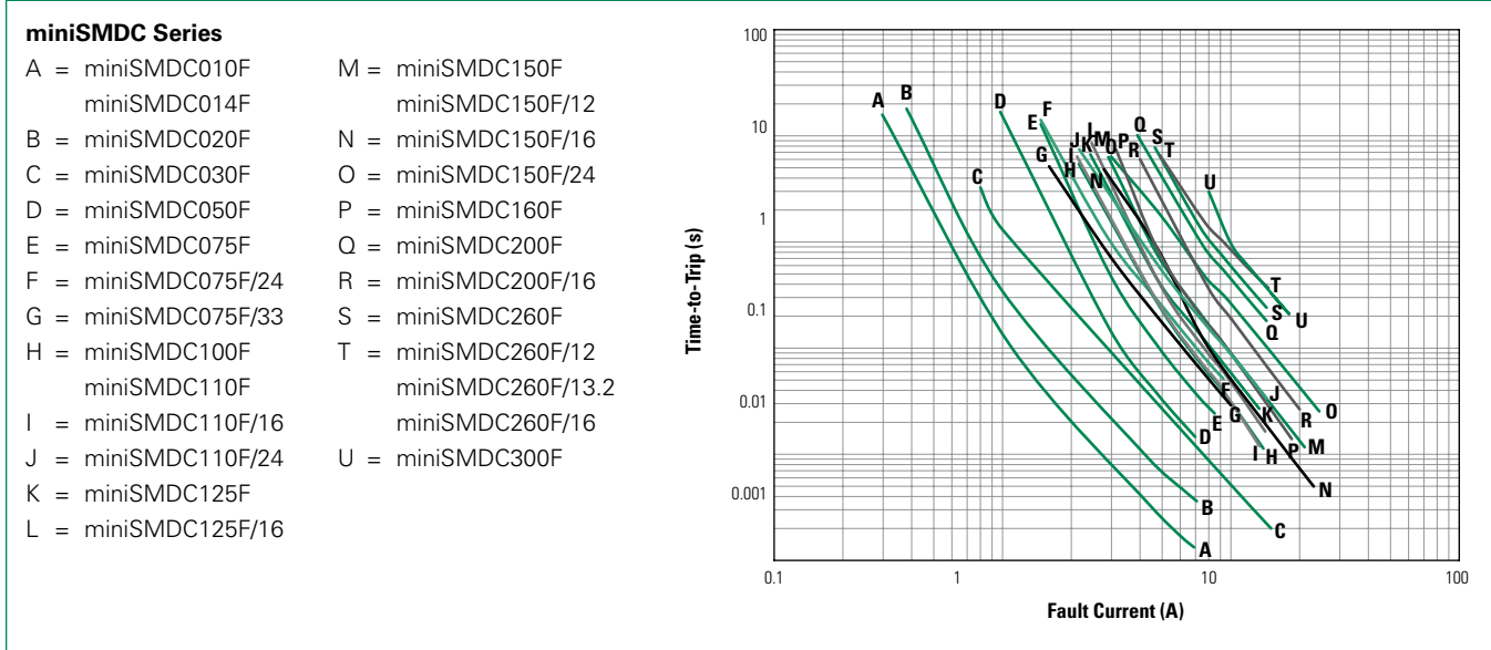
Typical Time-to-Trip Curves at 20°C
