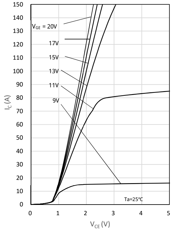
Fig. 2 Output characteristics
