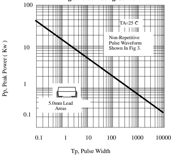
Fig. 5 Pulse Rating Curve
