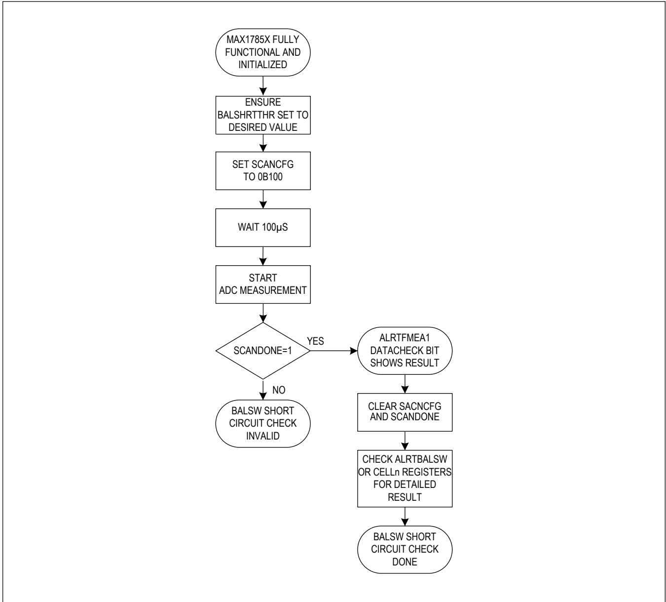
Figure 103. BALS SW Short Diagnostic Chart
