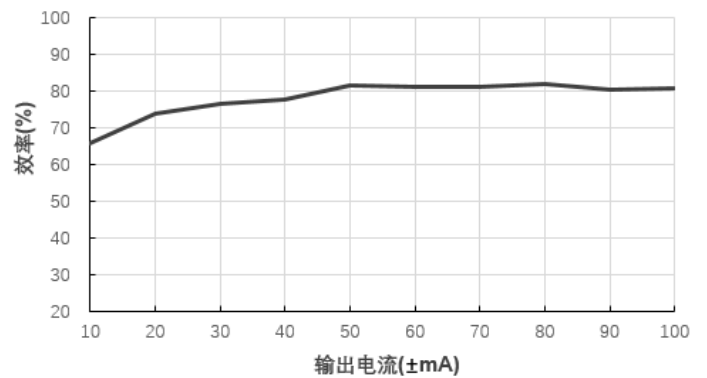
效率Vs输出电流(Vin=12V)@E1215S-1WR3
