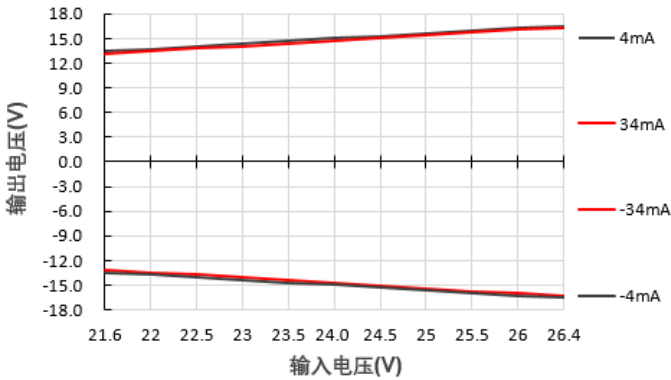
输出电压Vs输入电压@E2415S-1WR2
