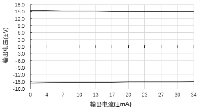
输出电压Vs输出电流(Vin=5V)@E0515S-1WR2
