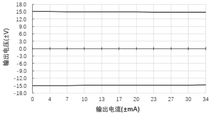
输出电压Vs输出电流(Vin=12V)@E2415S-1WR2
