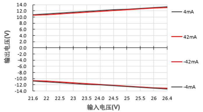
输出电压Vs输入电压@E2412S-1WR2
