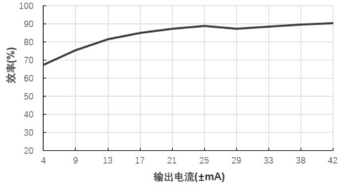
效率Vs输出电流(Vin=24V)@E2412S-1WR2
