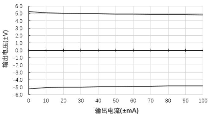
输出电压Vs输出电流(Vin=12V)@E2405S-1WR2
