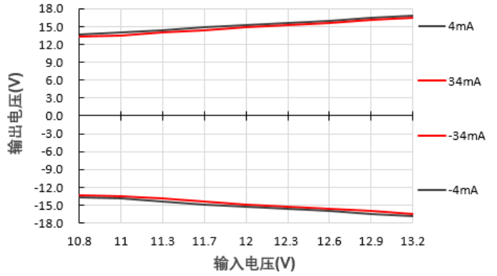
输出电压Vs输入电压@E1215S-1WR2
