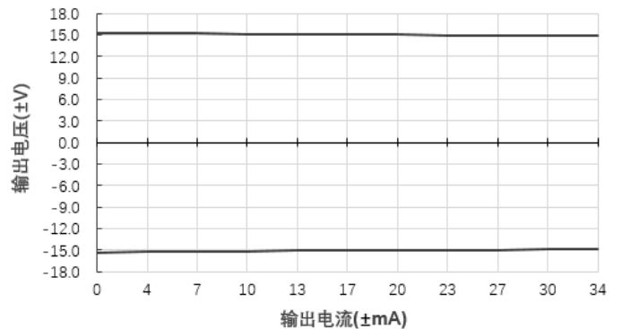
输出电压Vs输出电流(Vin=12V)@E1215S-1WR2
