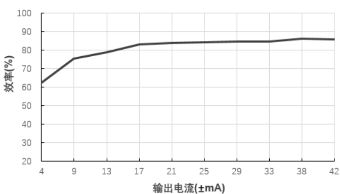
效率Vs输出电流(Vin=12V)@E1212S-1WR2
