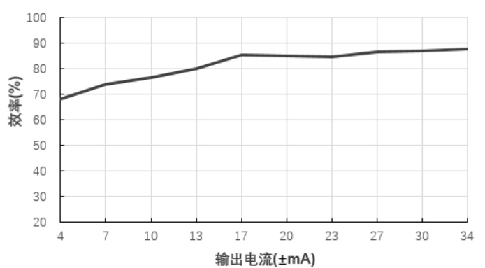
效率Vs输出电流(Vin=12V)@E1215S-1WR2
