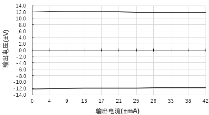
输出电压Vs输出电流(Vin=12V)@E1212S-1WR2
