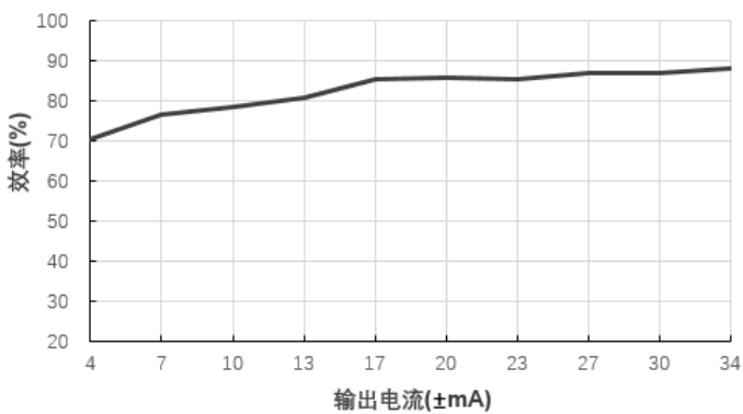
效率Vs输出电流(Vin=12V)@E1212S-1WR2
