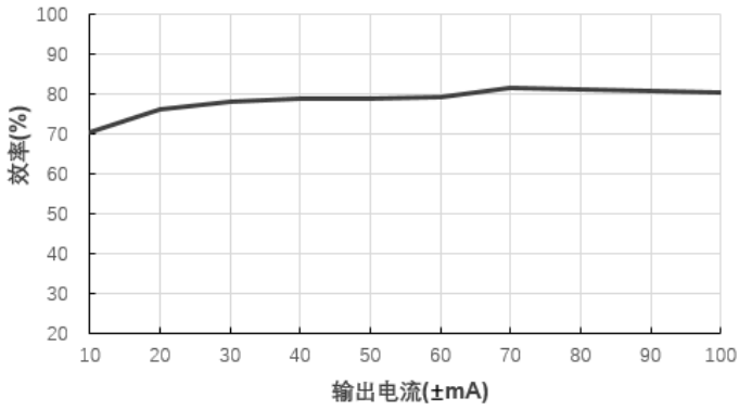
效率Vs输出电流(Vin=24V)@E2405S-1WR2
