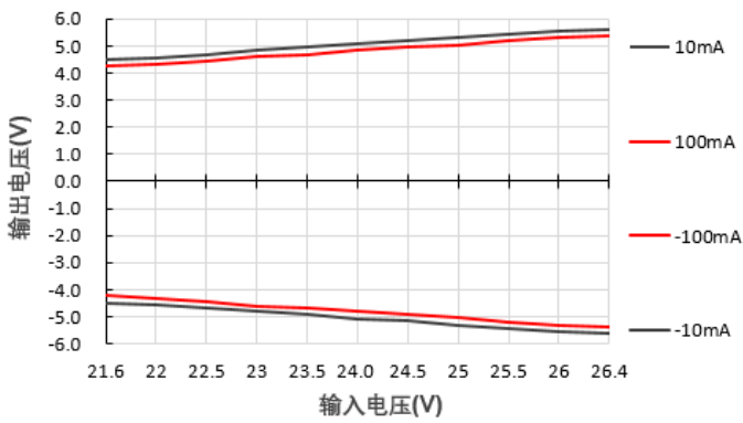
输出电压Vs输入电压@E2405S-1WR2
