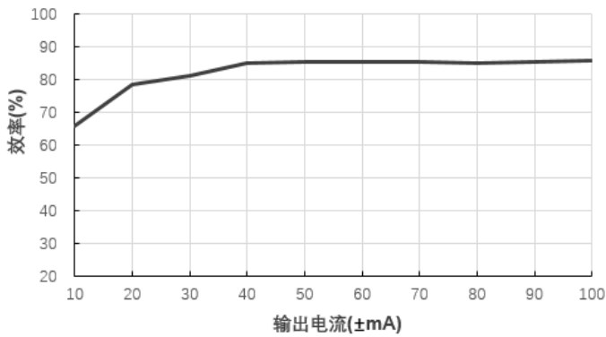
效率Vs输出电流(Vin=5V)@E0505S-1WR2
