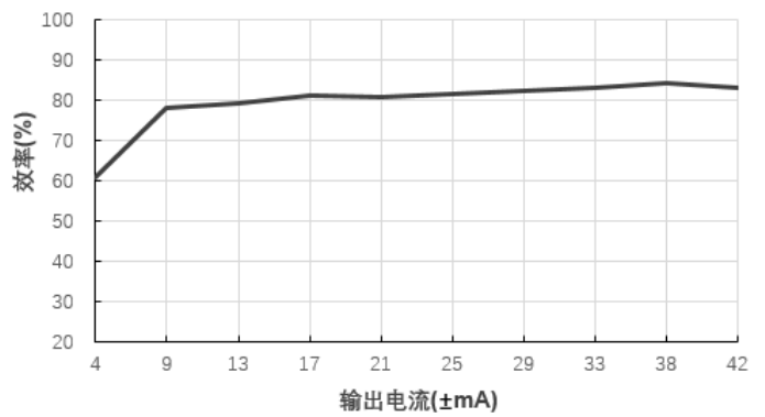
效率Vs输出电流(Vin=5V)@E0512S-1WR2
