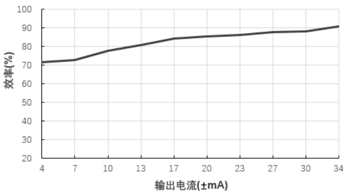
效率Vs输出电流(Vin=24V)@E2415S-1WR2
