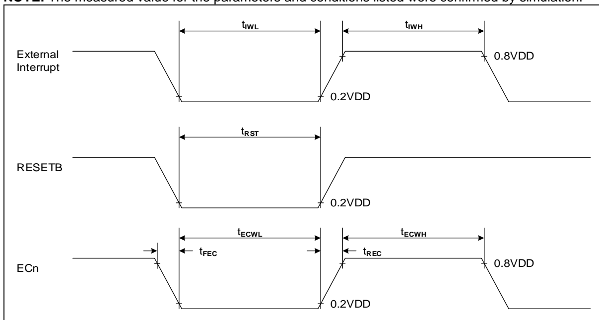
Figure 24. AC Timing
