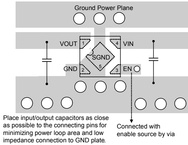
Figure 5. PCB Layout Guide for ZQFN-4L 1x1 package
