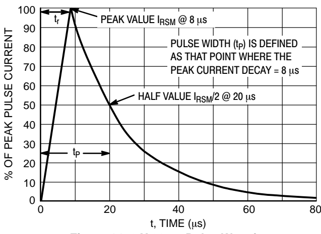
Figure 14. 8 X 20 \mu s Pulse Waveform
