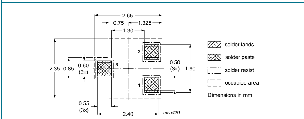
Fig 18. Reflow soldering footprint BAV70W (SOT323/SC-70)
