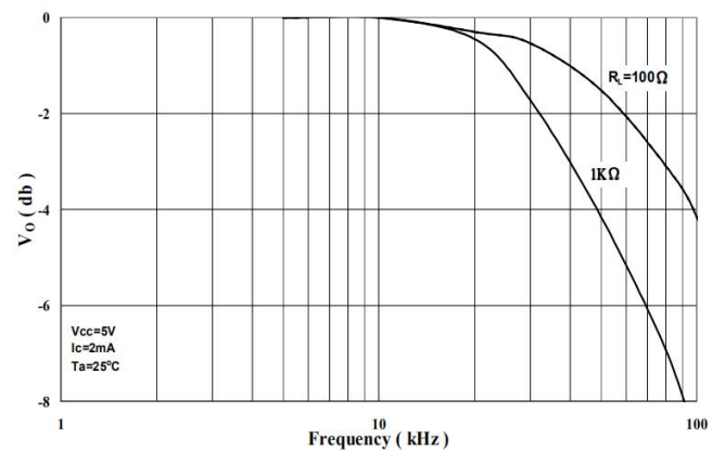
Figure 18. Frequency Response
