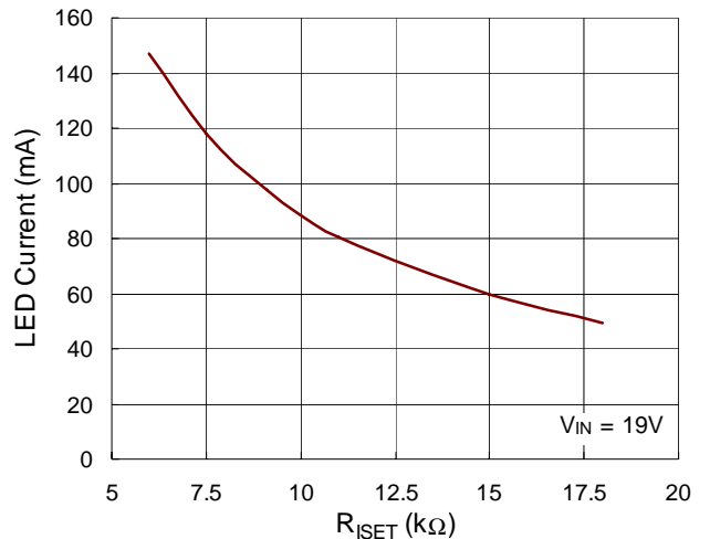
LED Current vs. R ISSET
