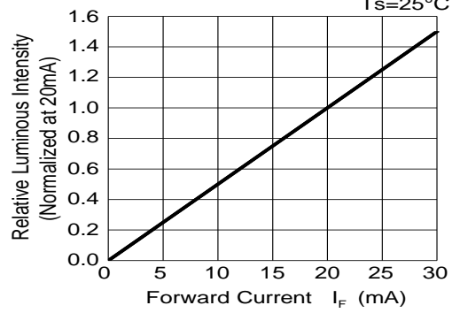
Fig.2-Relative Luminous Intensity vs. Forward Current Ts=25°C
