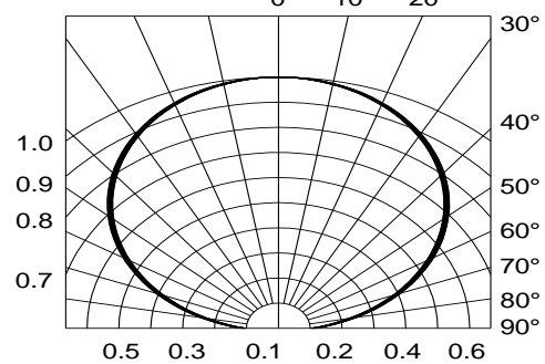
Fig.6-Radiation Diagram Ta=25°C
