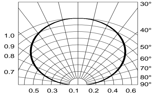
Fig.6-Radiation Diagram Ta=25°C
