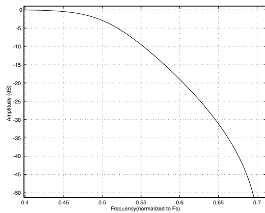
Figure 33. DAC Quad-Speed Transition Band (detail)
