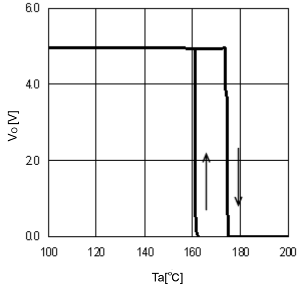
Fig.28 TSD ( I_o=0mA )
