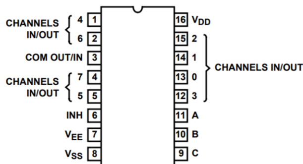
DIP16/SOP16/TSSOP16
